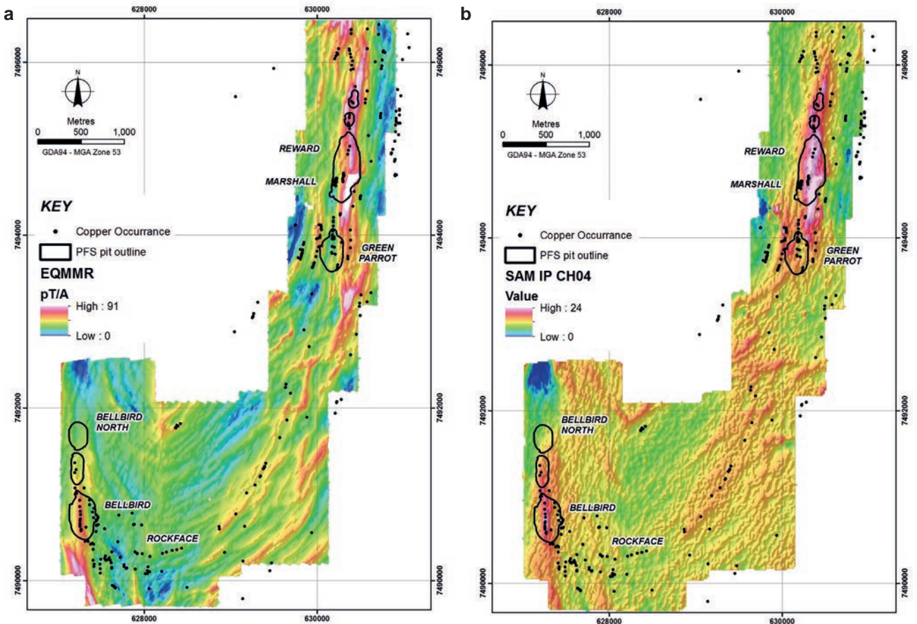
Figure 4. (a) SAM TFM. (b) SAM TFMIP.
