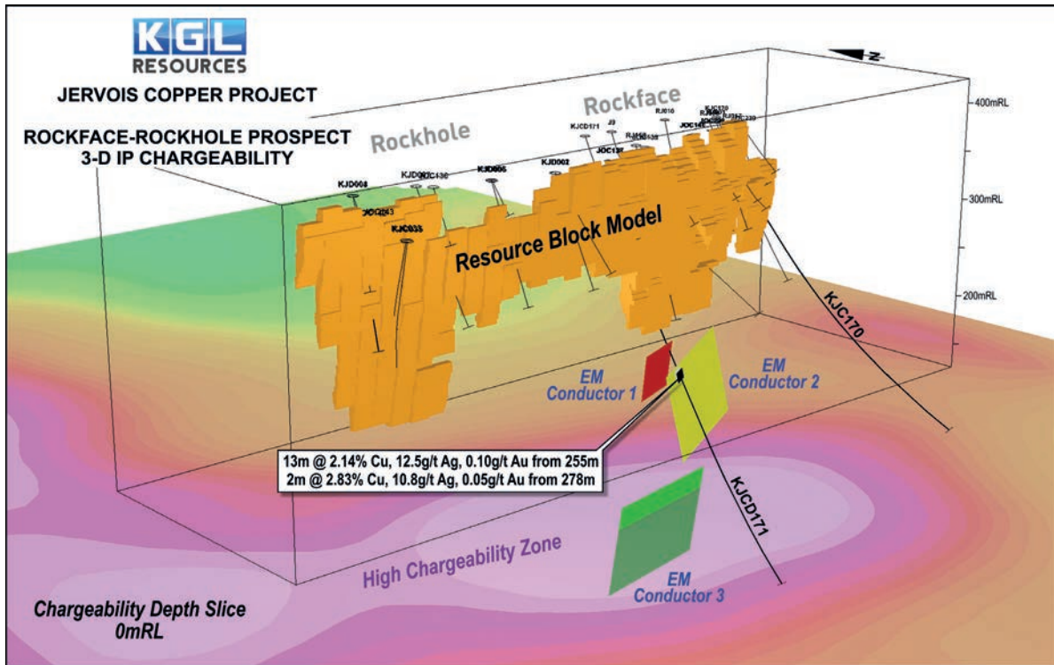
Figure 5. Rockface DHEM modelled conductive plates.
